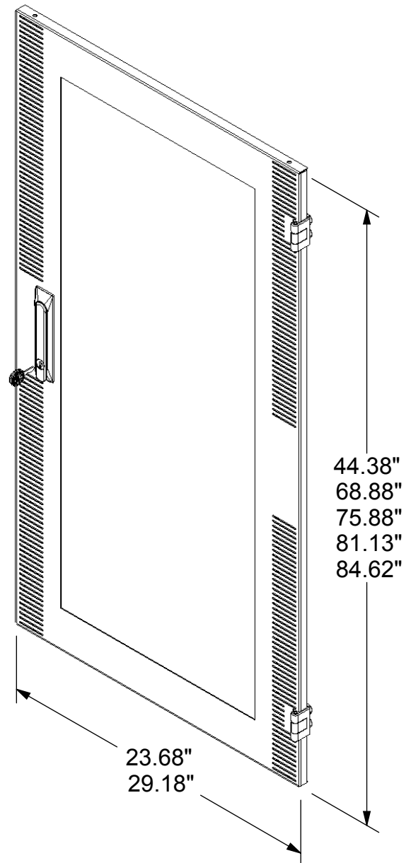
VENTED ACRYLIC DOOR, L w/SWING SINGLE LOCK SHOWN HERE
